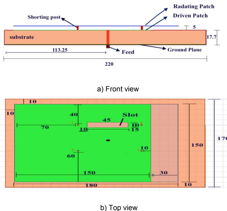
Fig. 2 – Viewing sides and dimensions of proposed tag antenna
